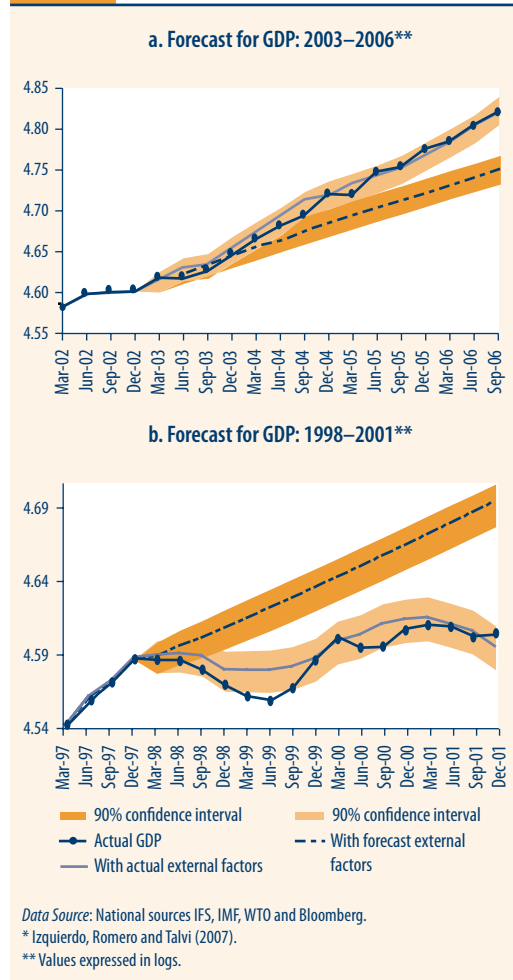
FIGURE 3 GDP Forecasts Conditional on External Variables: Bonanza vs. Crisis*
